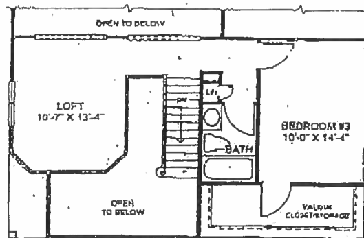
OPTIONAL SECOND FLOOR
